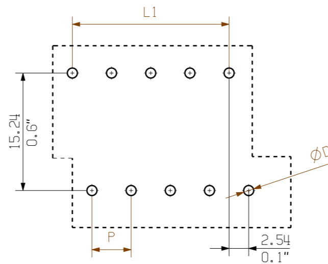
PCB LAYOUT
