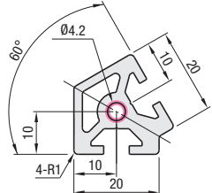
HFS60A5-20
