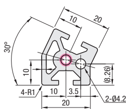
HFS30A5-20
