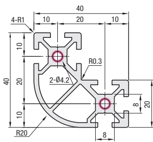
HFSR5-404020
