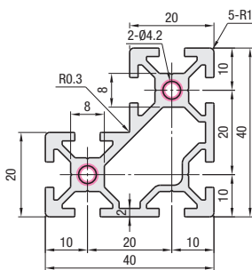
HFS5-404020
