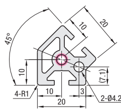
HFS45A5-20
