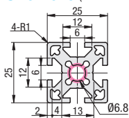
NFS5-2525 HFS5-2525
