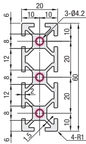
NFS5-2060 HFS5-2060
