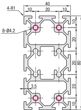
NFS5-4080 HFS5-4080
