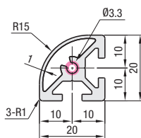
HFSR5-2020
