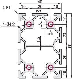
NFS5-4060 HFS5-4060
