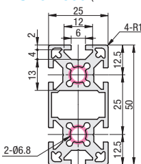
NFS5-2550 HFS5-2550
