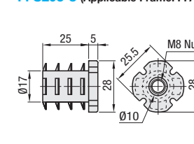
■ Insert Nut M8 FFS203-8 (Applicable Frame: FFA28)
