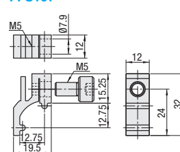
■ Panel Holder FFS107
