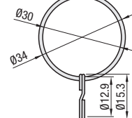
■ Ring Slider FFS106 (Set of 10)
