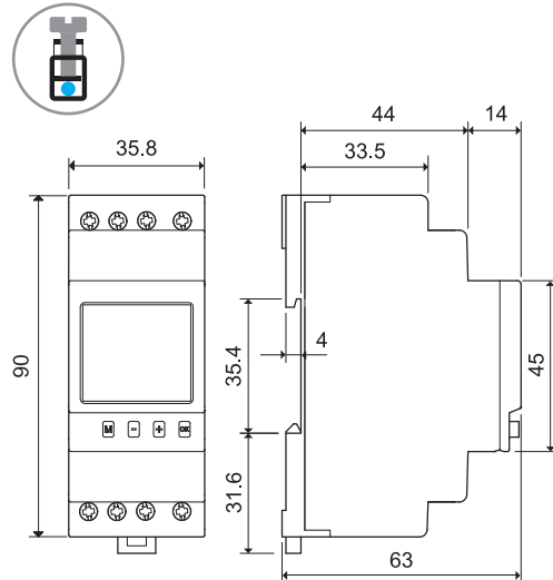
12.51/12.81 Screw terminal
