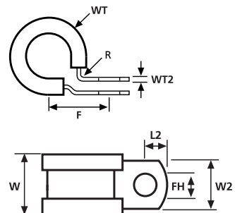
Aluminium P Clips with a Chloroprene insert
