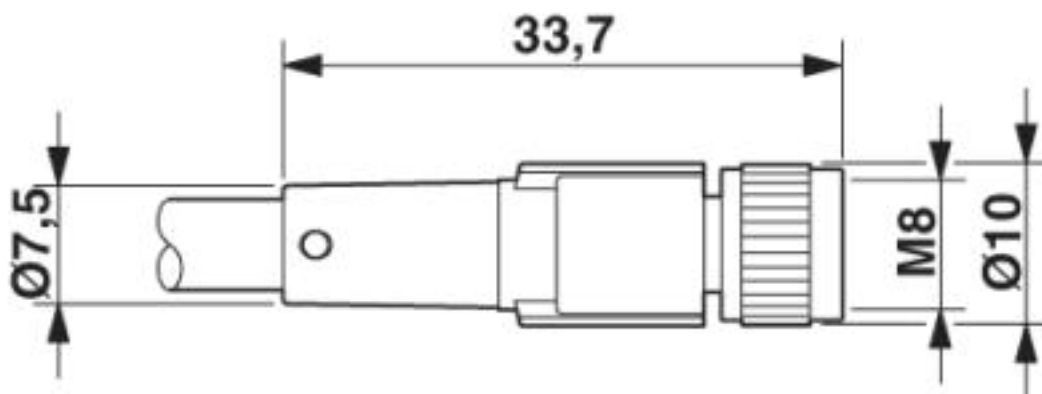
Socket M8 x 1, straight
