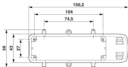
Dimensional drawing top view
