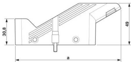
Dimensional drawing, a = 150.2 mm
