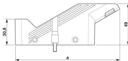
Dimensional drawing, a = 123.7
