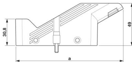
Dimensional drawing, a = 103.2
