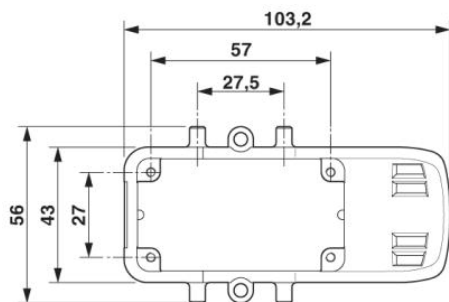
Dimensional drawing top view
