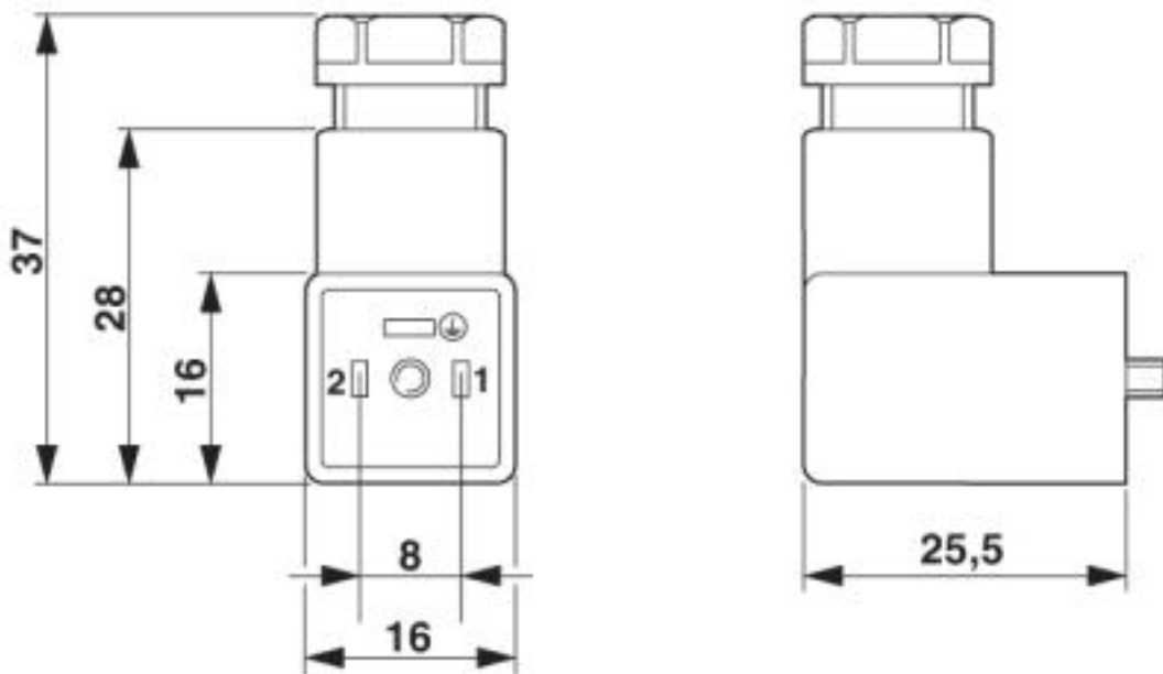
Dimensioned drawing
