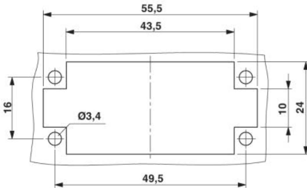
Panel cutout
