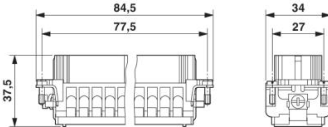
Female insert
