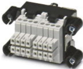
Contact insert set for sleeve side, sleeve frame with PE, 4 fixing screws, 8-pos. contact inserts preassembled, 6 coding profiles
