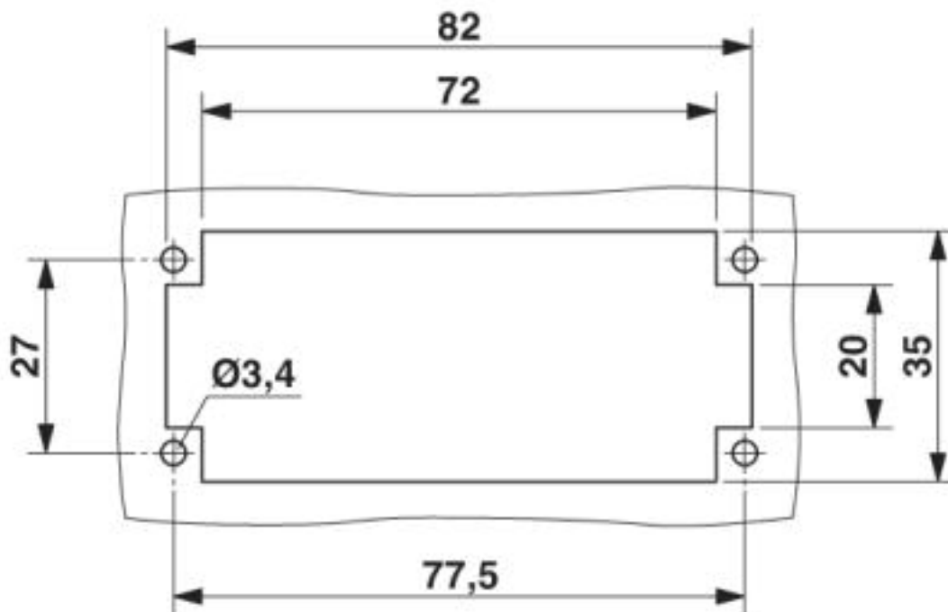
Panel cutout
