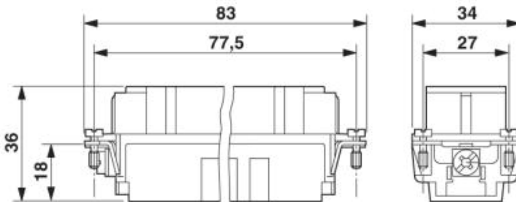
Female insert
