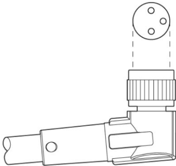
Layout of connector pin assignments
