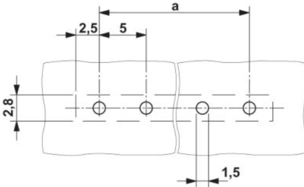
Drilling diagram
