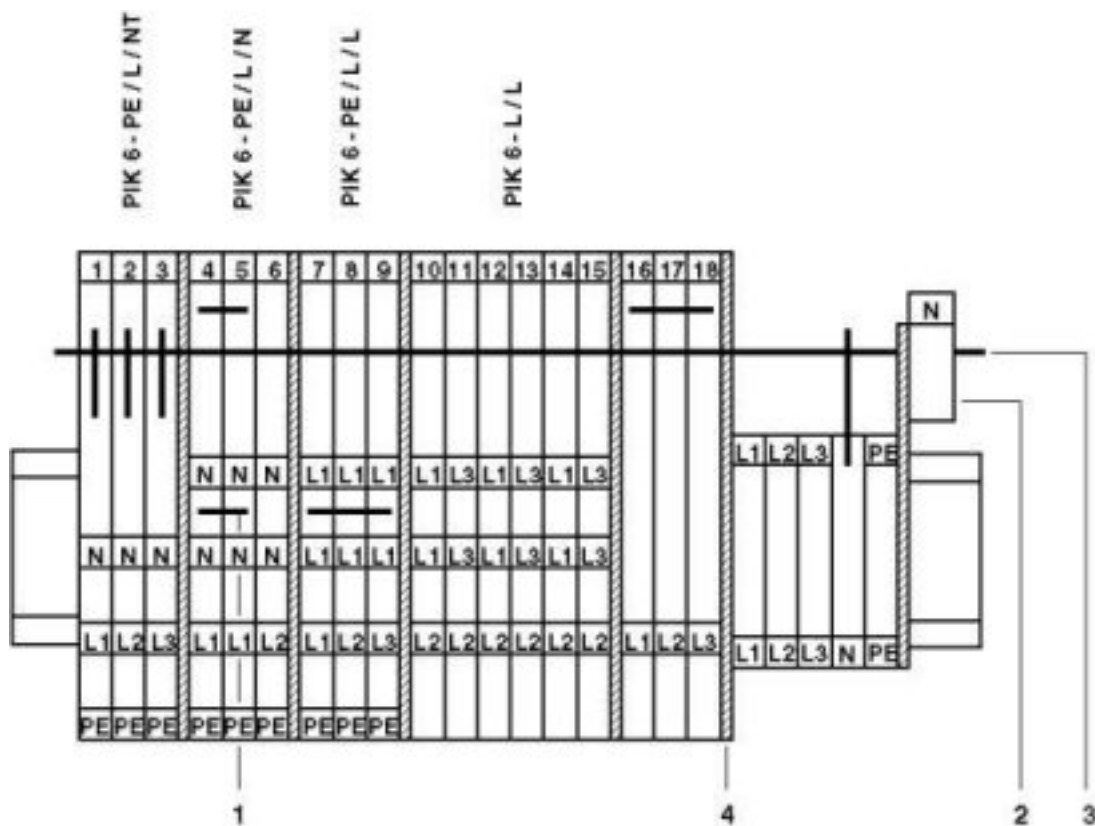
Circuit diagram
