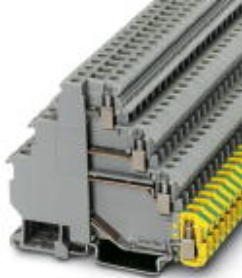
Sensor/actuator terminal block, Cross section: 0.2 mm 2 - 4 mm 2 , AWG: 24 - 12, Connection type: Screw connection, Width: 6.2 mm, Color: gray, Mounting type: NS 35/7,5, NS 35/15
